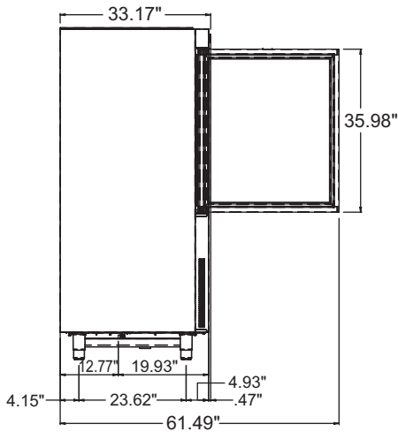
NBCF99/59-8A SIDE VIEW
