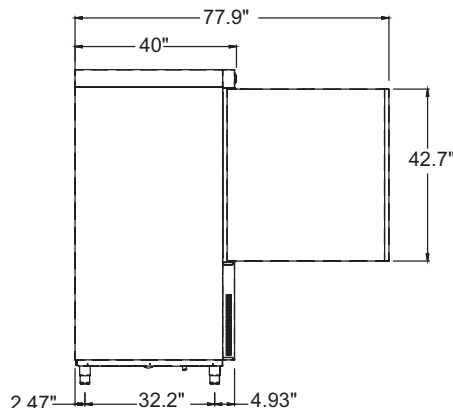
NBCF115/55-16A NBCF220/110-16A SIDE VIEW
