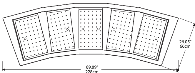
N8094-R Plan View
