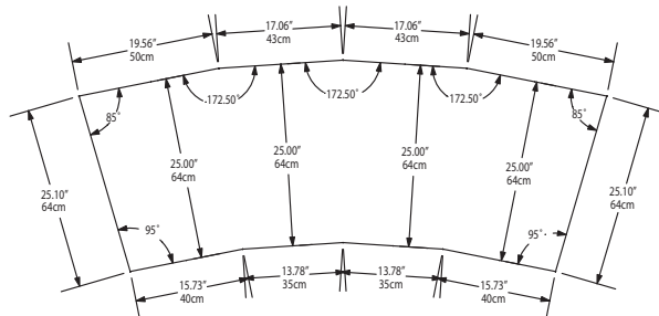
N8076-R Cutout Dimensions
