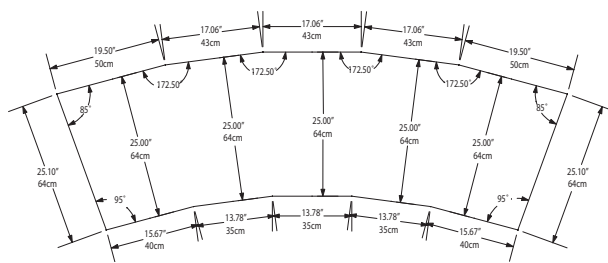
N8094-R Cutout Dimensions
