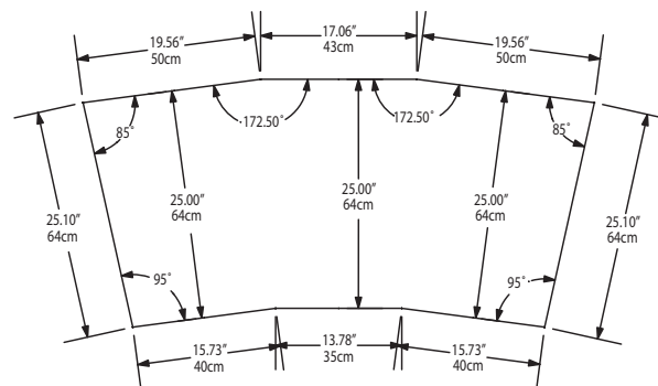
N8059-R Cutout Dimensions
