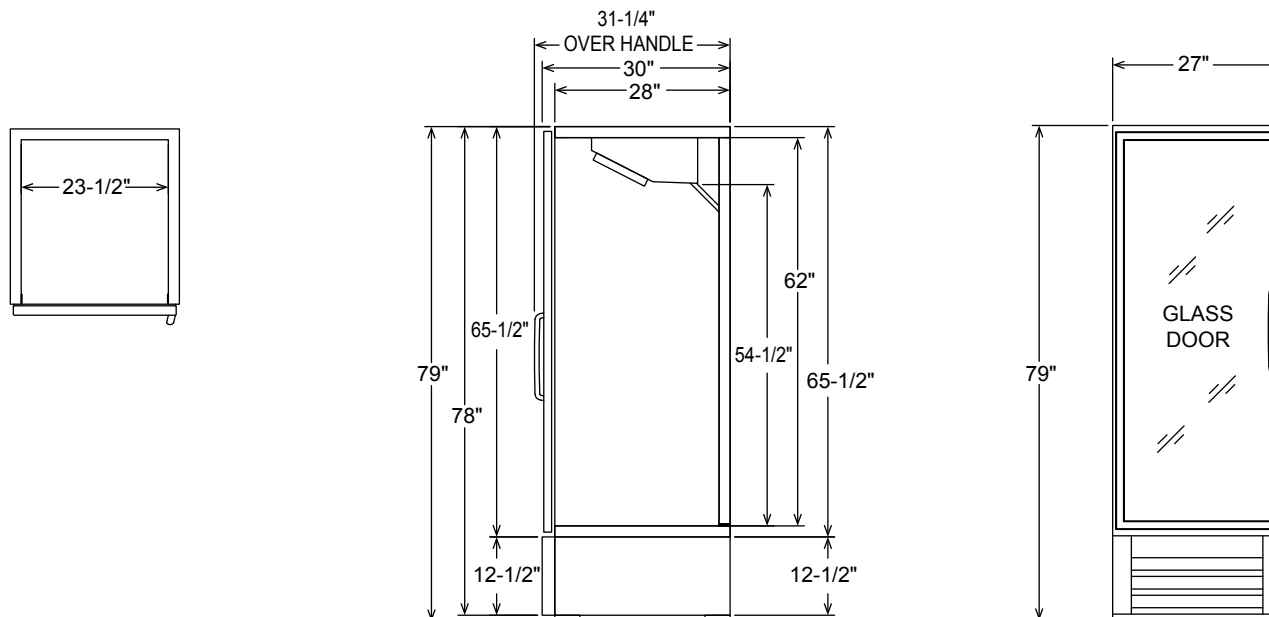
PLAN VIEW
