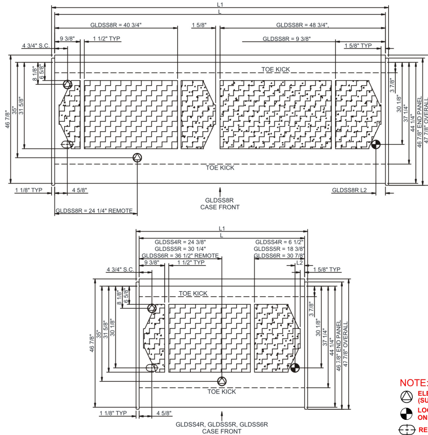
PLAN VIEW
