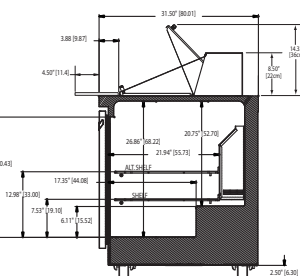
4460N-18M Right Side View
