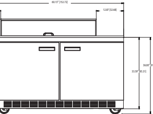
4460N-18M Elevation View
