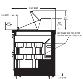
D4460N-12M Right Side View
