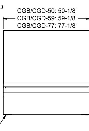
ELEVATION VIEW
