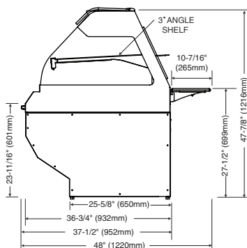
ED2SYS-72/2S Profile
