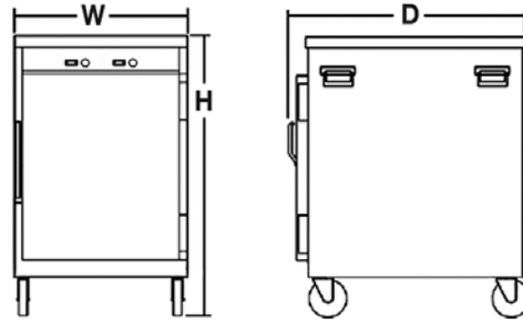
VHU7 Front &amp; Side Views
