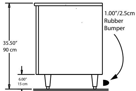
End View Models UC4048P
