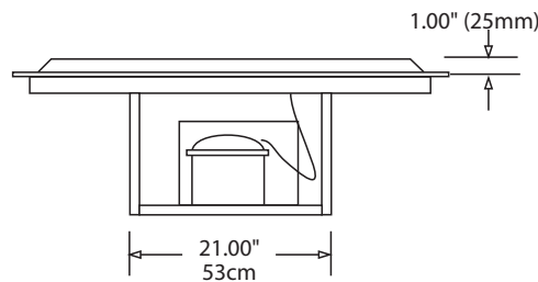
Elevation View N8200P Models
