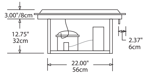
Right End View N8200P Models
