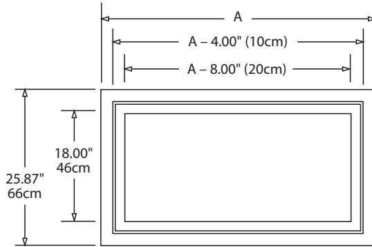
Plan View N8200P Models
