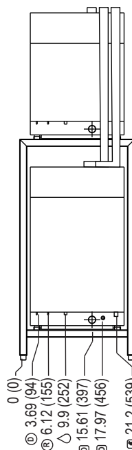
REAR VIEW
