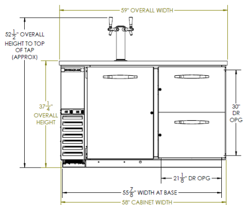
Elevation View
