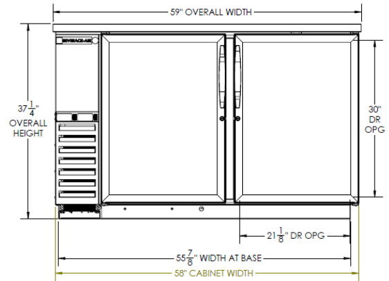
Elevation View
