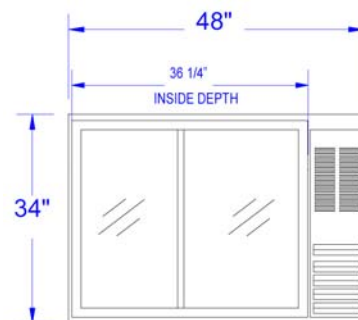
FRONT BB48GSY-1-B
