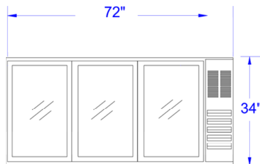
FRONT BB72GSY-1-B
