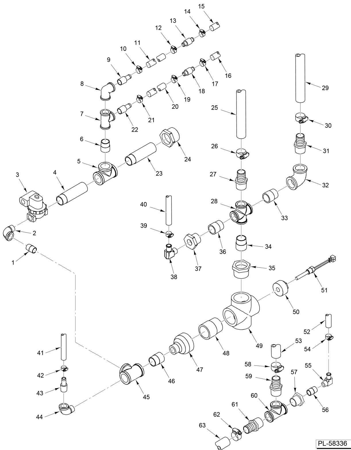
DRAIN ASSEMBLY (CURRENT CONSTRUCTION)
