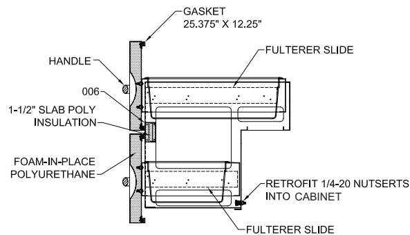
SIDE SECTION
