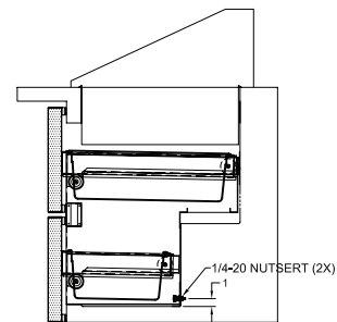
SECTION OF TYP. CABINET w/ DRAWERS
