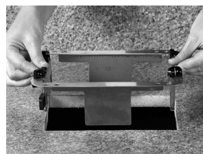
5. Insert the mounting adapter (B) into the hole making sure the retainer paddles (C) are folded flat against the mounting adapter.
