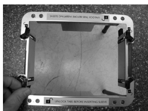
7. The black thumbscrews (D) must be turned as shown above in order for the dispenser to seat properly into the mounting adapter. Refer to printed info/ icons on adapter flange.
