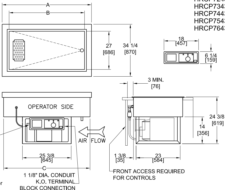
PRODUCT DIMENSIONS INCHES [MM]
