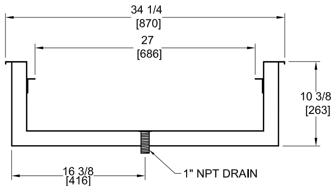
CROSS-SECTION OF HOT & COLD PAN
