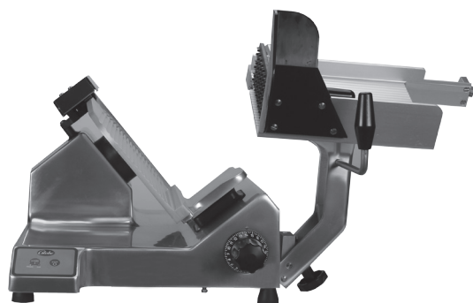
Figure 12-2 Cleaning Position
