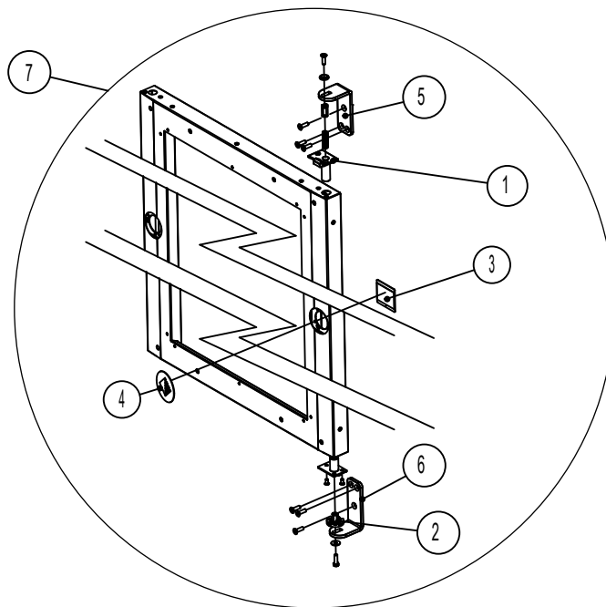
LEFT HAND TO RIGHT HAND HINGE
