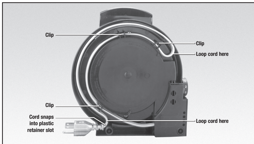
Figure 7. Cord clips under base. WaffleCone Express™ stores upright as shown.
