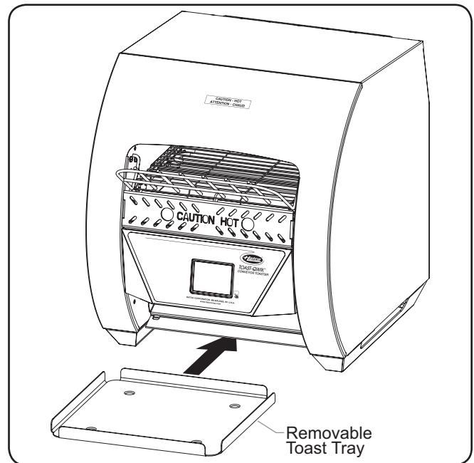
Installing the Toast Tray (Model TQ3-400 only)
