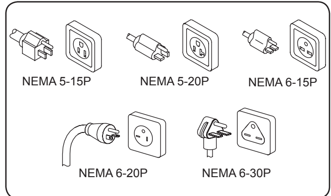
Plug Configurations
