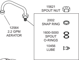
19119 SWIVEL SPOUT RETRO-FIT KIT
