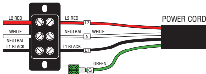
120/208-240V 3 WIRE + GROUND
