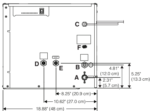
Side view — air-cooled and water-cooled
