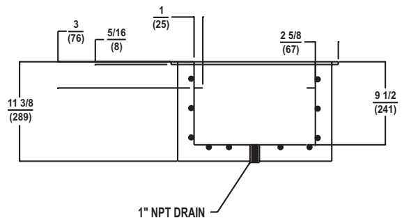
CROSS-SECTION OF COLD PAN
